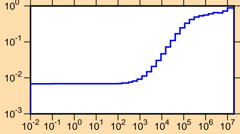
\mu vs. E for ^{114}\text{Sb}(\text{mt251})
