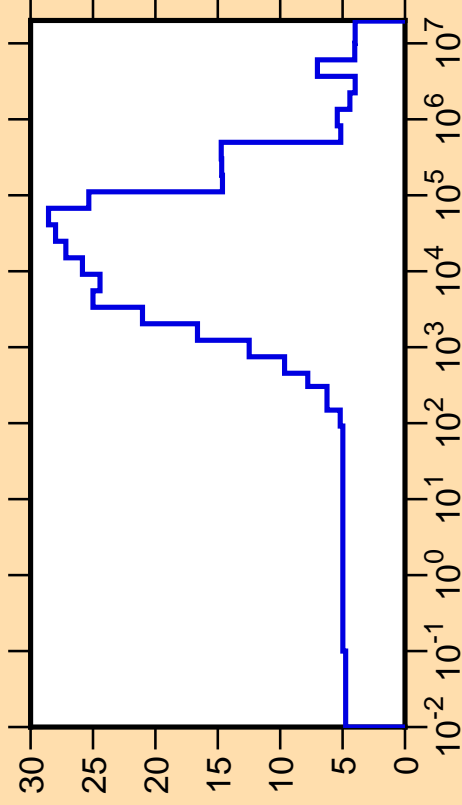
\Delta\mu/\mu vs. E for ^{114}\text{Sb}(\text{mt251})
