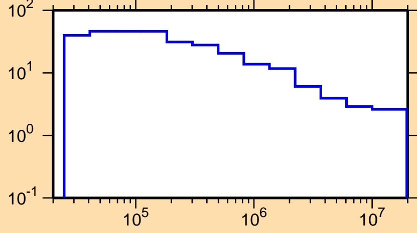
\Delta\sigma/\sigma vs. E for ^{114}\text{Sb}(n,\text{nonel.})
