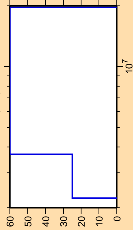
\Delta\sigma/\sigma vs. E for ^{114}\text{Sb}(n,d)
