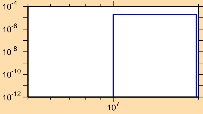
\sigma vs. E for ^{114}\text{Sb}(n,nd)
