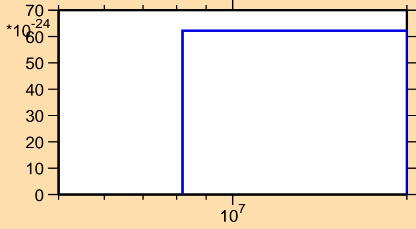
\sigma vs. E for ^{114}\text{Sb}(\text{mt } 11)
