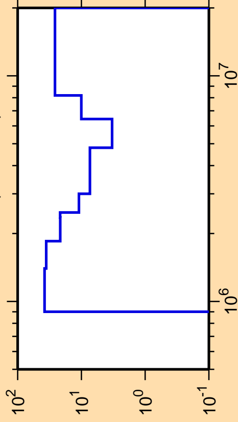
\Delta\sigma/\sigma vs. E for ^{114}\text{Sb}(n,\text{ncont.})
