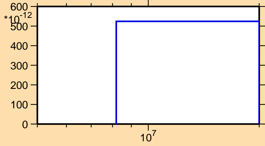
\sigma vs. E for ^{114}\text{Sb}(n,\text{pd})
