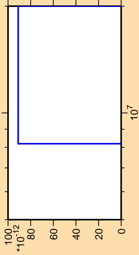
\Delta\sigma/\sigma vs. E for ^{114}\text{Sb}(\text{mt } 11)
