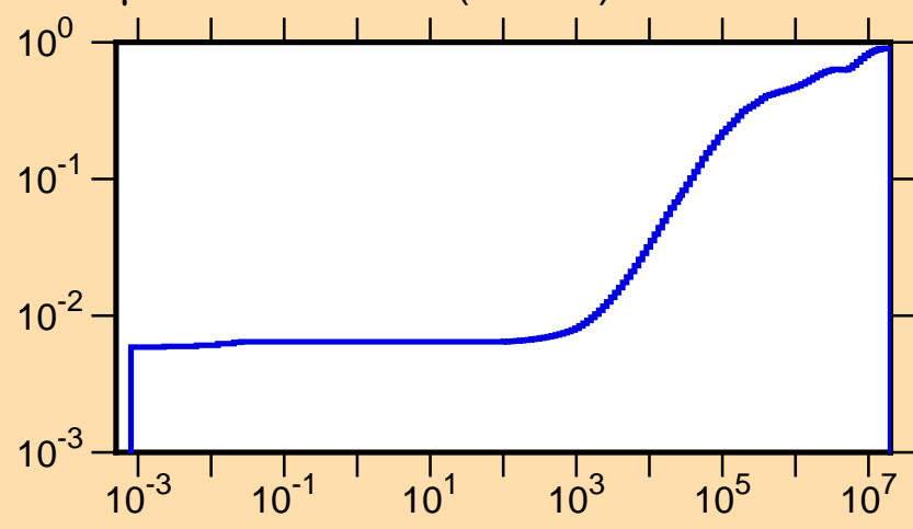
\mu vs. E for ^{115}\text{Sb}(\text{mt251})
