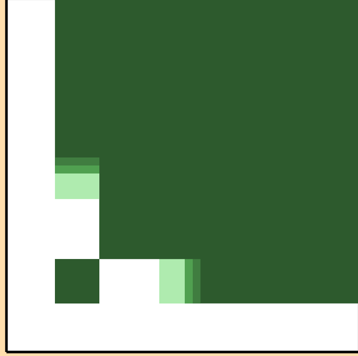
\sigma vs. E for ^{116}\text{Sb}(n,2np)
