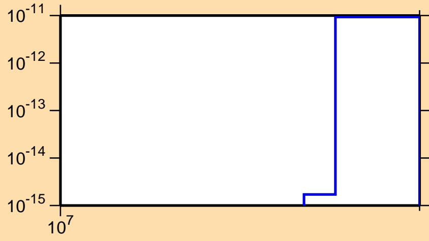
\sigma vs. E for ^{116}\text{Sb} (mt 34)
