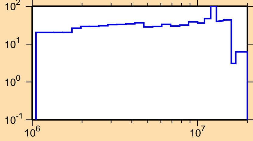
\Delta\sigma/\sigma vs. E for ^{116}\text{Sb}(n,n_1)
