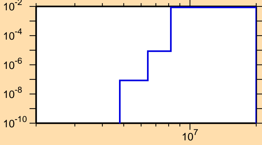
\sigma vs. E for ^{116}\text{Sb}(n,d)
