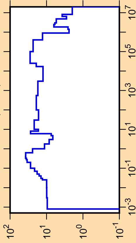
\Delta\sigma/\sigma vs. E for ^{116}\text{Sb}(n,\text{tot.})
