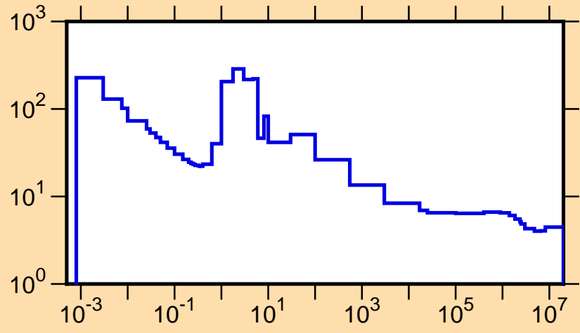
\sigma vs. E for ^{116}\text{Sb}(n,\text{tot.})
