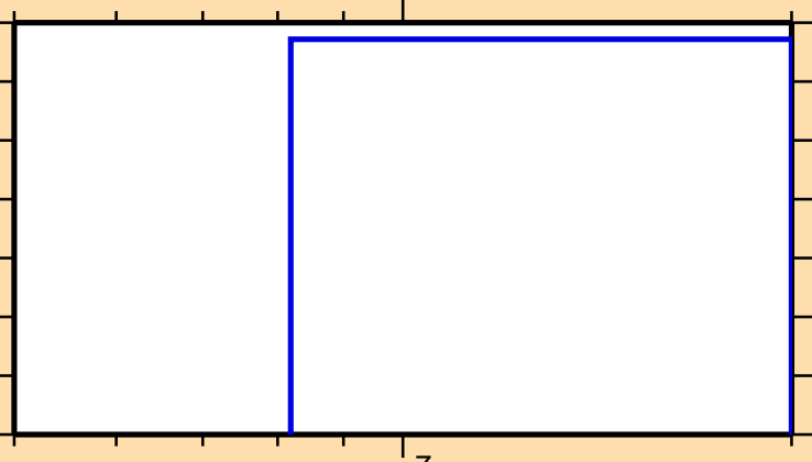
\sigma vs. E for ^{116}\text{Sb}(n,\text{nd})
