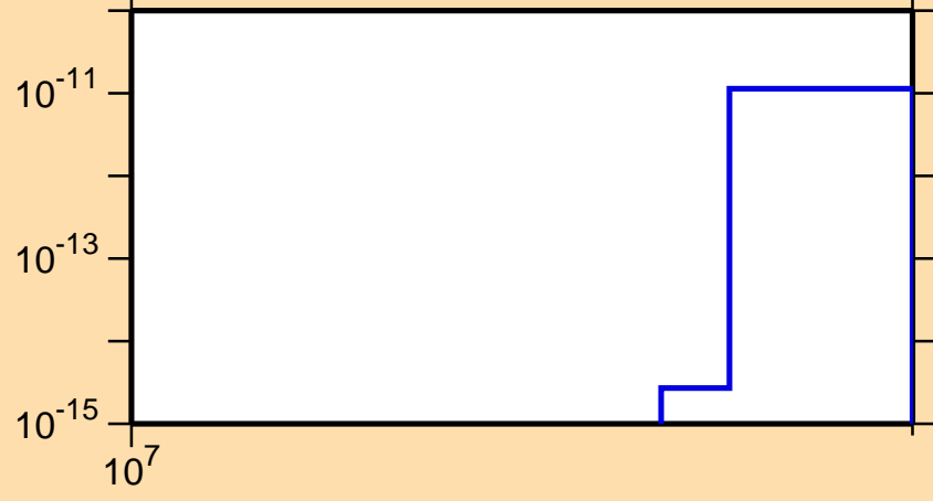
\sigma vs. E for ^{116}\text{Sb} (mt 34)
