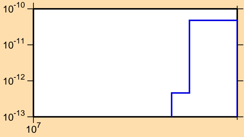
\sigma vs. E for ^{116}\text{Sb} (mt 45)
