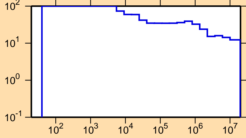
\Delta\sigma/\sigma vs. E for ^{116}\text{Sb}(n,\text{nonel.})
