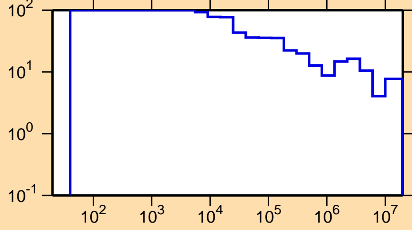
\Delta\sigma/\sigma vs. E for ^{116}\text{Sb}(n,\text{tot.})
