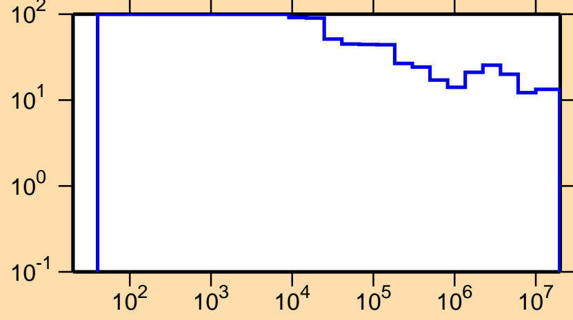
\Delta\sigma/\sigma vs. E for ^{116}\text{Sb}(n,\text{el.})
