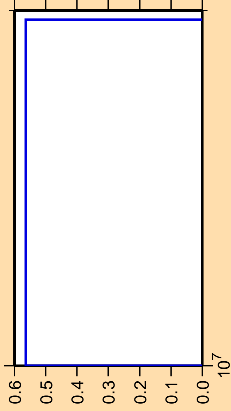
\Delta\sigma/\sigma vs. E for ^{116}\text{Sb} (mt 34)
