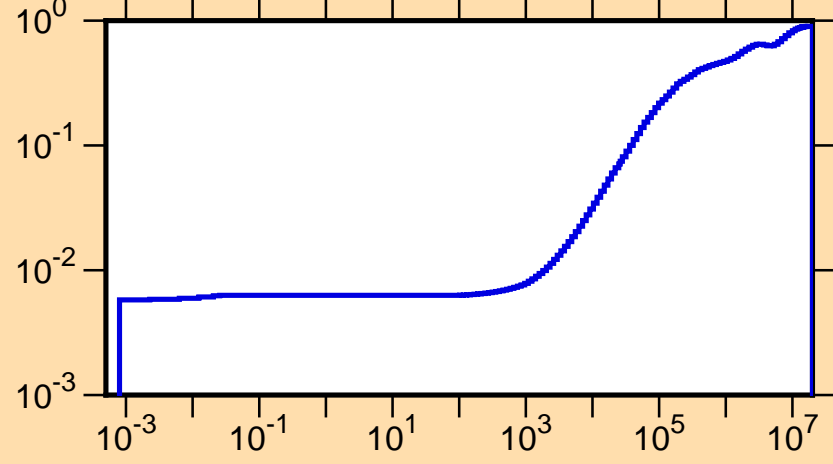
\mu vs. E for ^{117}\text{Sb}(\text{mt251})
