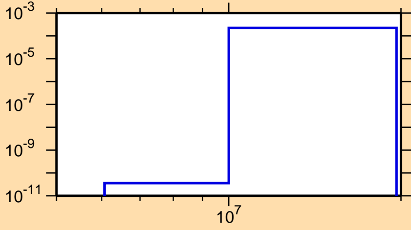
\sigma vs. E for ^{117}\text{Sb}(n,t)
