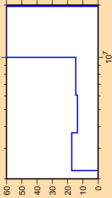
\Delta\sigma/\sigma vs. E for ^{117}\text{Sb}(n,\text{ncont.})
