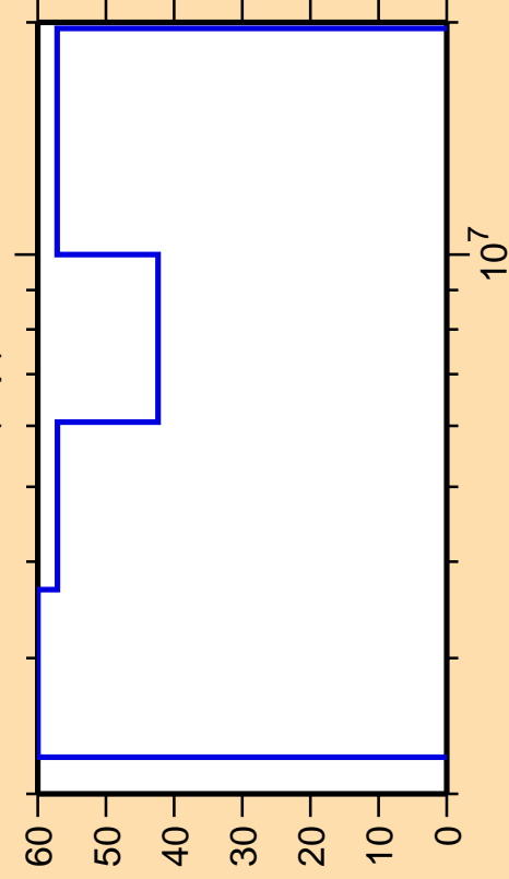
\Delta\sigma/\sigma vs. E for ^{117}\text{Sb}(n,p)
