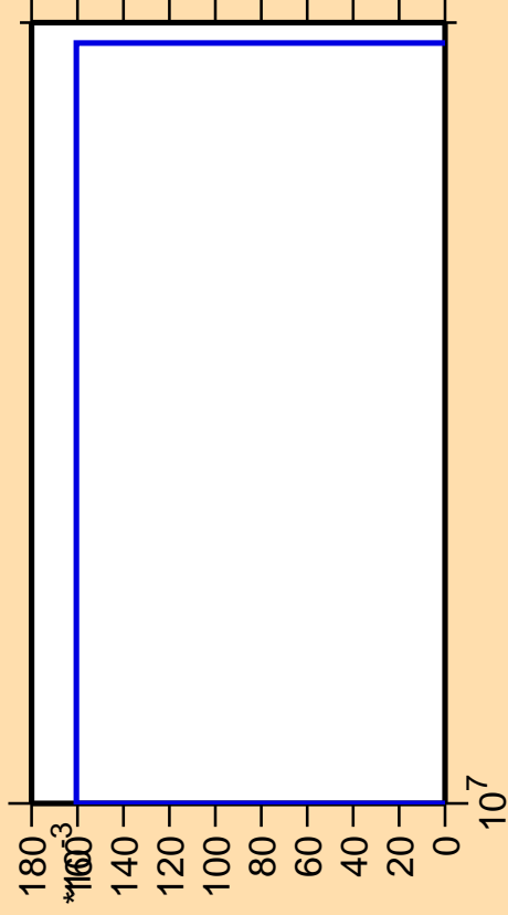
\Delta\sigma/\sigma vs. E for ^{117}\text{Sb}(n,\text{pd})
