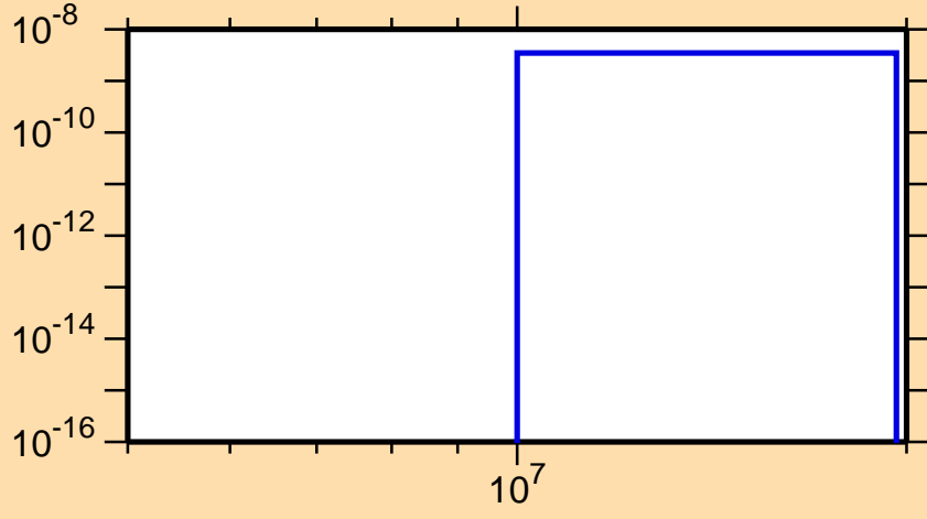
\sigma vs. E for ^{117}\text{Sb}(n,p\alpha)
