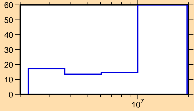
\Delta\sigma/\sigma vs. E for ^{117}\text{Sb}(n,ncont.)
