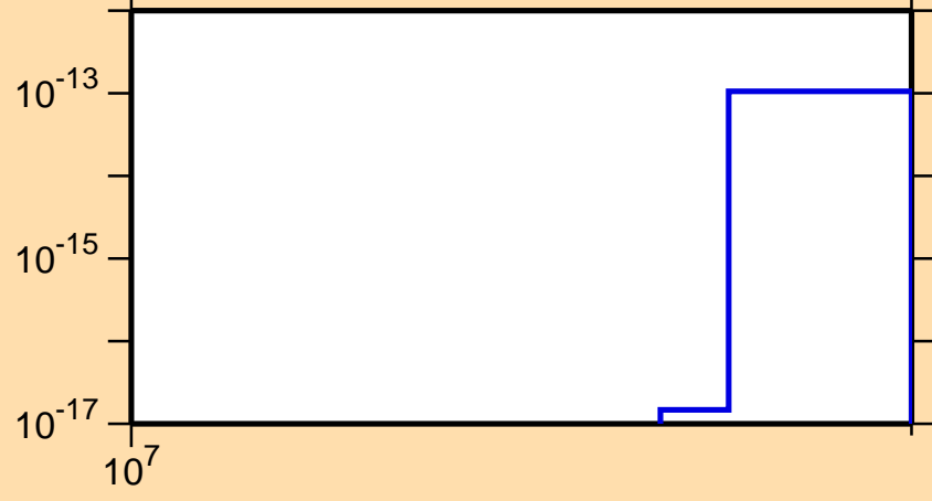
\sigma vs. E for ^{118}\text{Sb}(n,pd)
