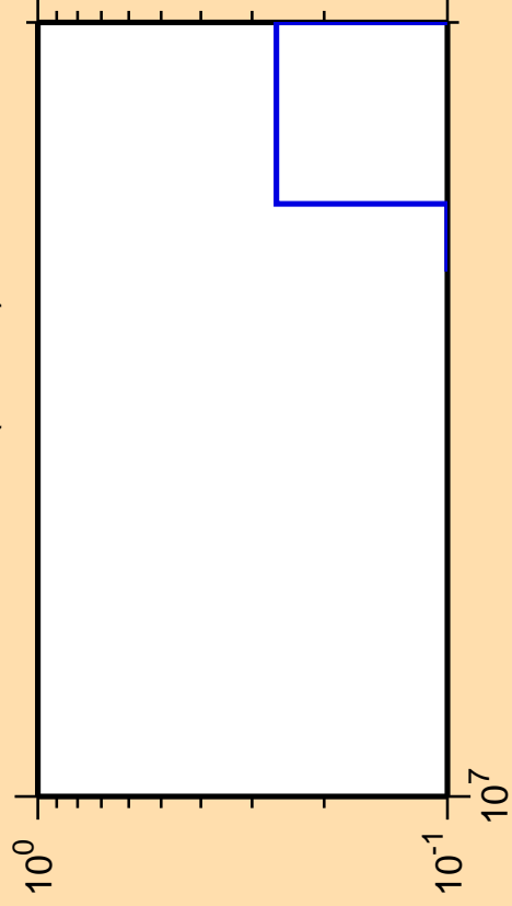
\Delta\sigma/\sigma vs. E for ^{118}\text{Sb} (mt 45)
