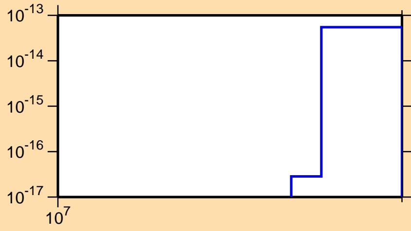
\sigma vs. E for ^{118}\text{Sb} (mt 45)
