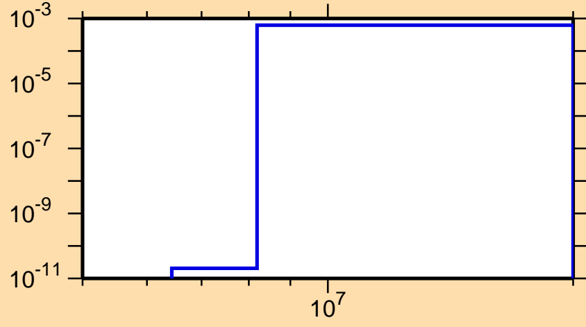
\sigma vs. E for ^{118}\text{Sb}(n,t)
