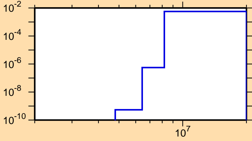
\sigma vs. E for ^{118}\text{Sb}(n,d)
