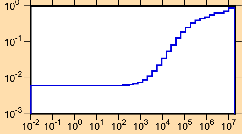
\mu vs. E for ^{119}\text{Sb}(\text{mt251})
