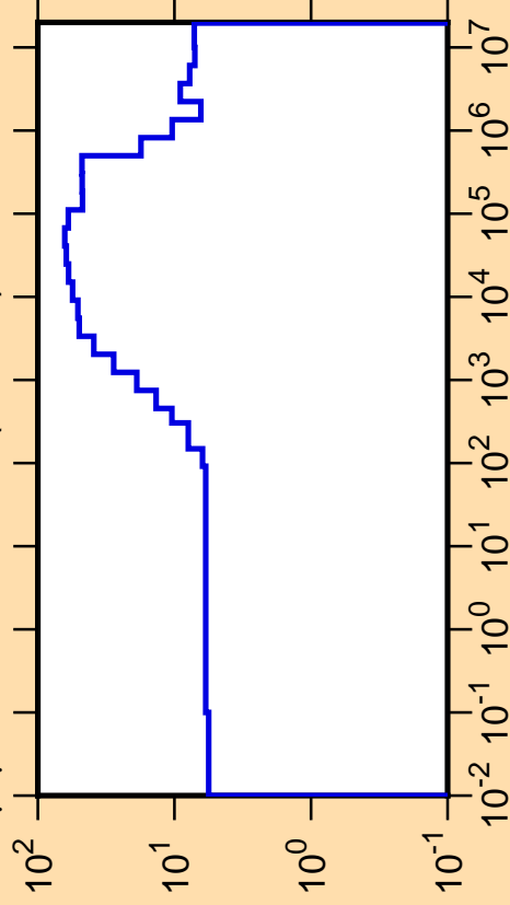
\Delta\mu/\mu vs. E for ^{119}\text{Sb}(\text{mt251})
