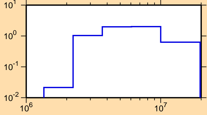
\sigma vs. E for ^{119}\text{Sb}(n,n\text{cont.})
