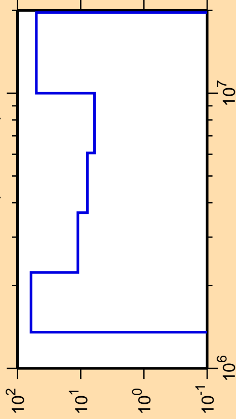
\Delta\sigma/\sigma vs. E for ^{119}\text{Sb}(n,\text{ncont.})
