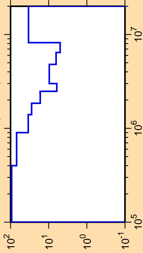
\Delta\sigma/\sigma vs. E for ^{119}\text{Sb}(n,\text{inel.})
