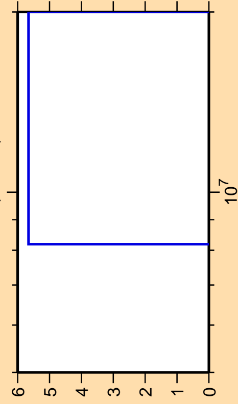
\Delta\sigma/\sigma vs. E for ^{119}\text{Sb}(n,2n\alpha)
