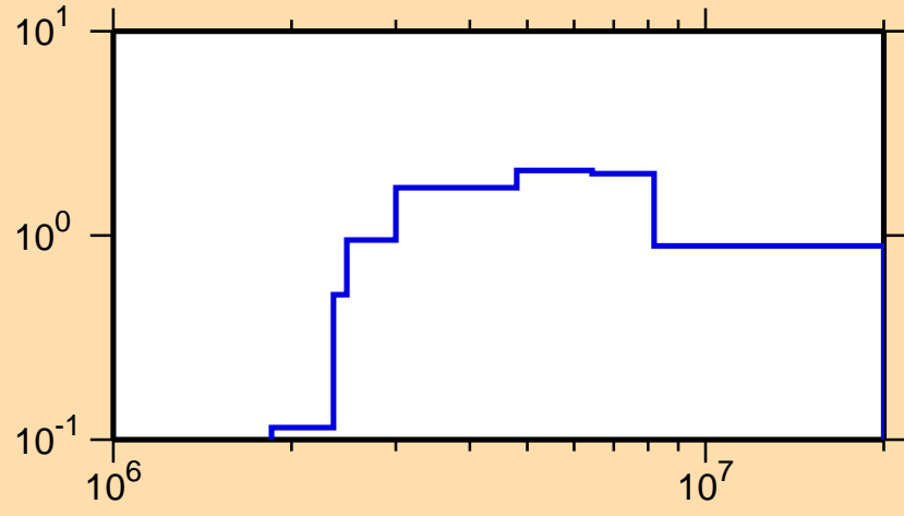
\sigma vs. E for ^{119}\text{Sb}(n,n\text{cont.})
