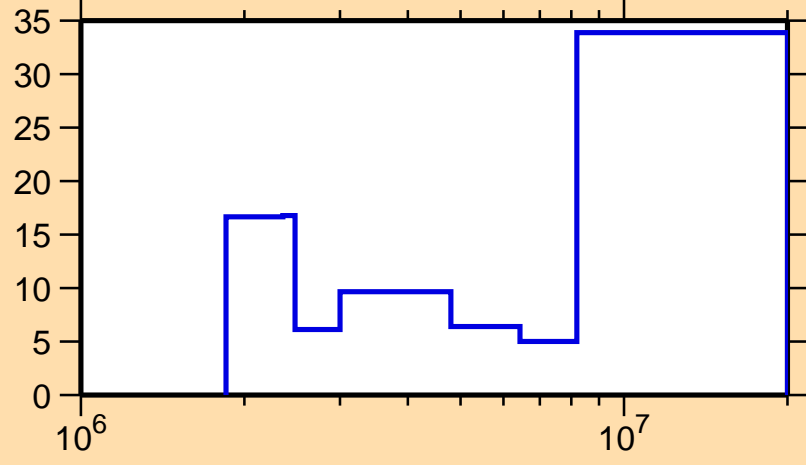
\Delta\sigma/\sigma vs. E for ^{119}\text{Sb}(n,inel.)
