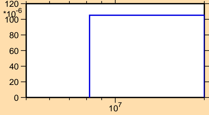
\sigma vs. E for ^{119}\text{Sb}(n,t)
