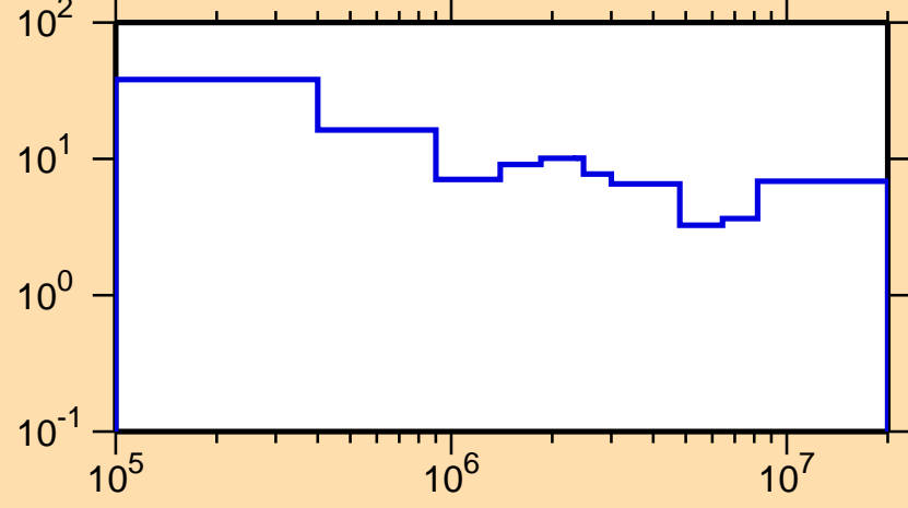
\Delta\sigma/\sigma vs. E for ^{119}\text{Sb}(n,\text{tot.})
