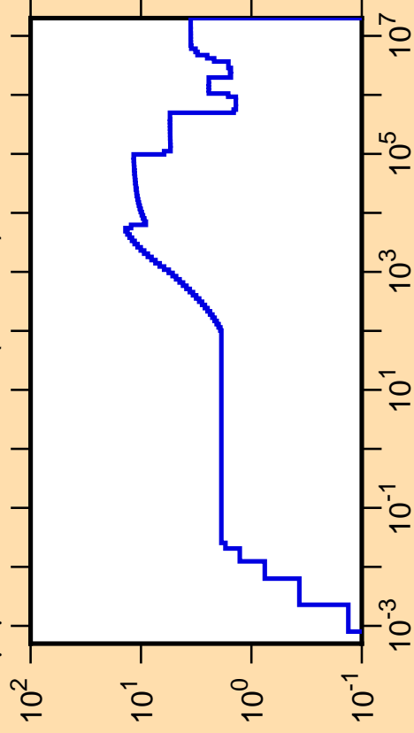
\Delta\mu/\mu vs. E for ^{120}\text{Sb}(\text{mt251})
