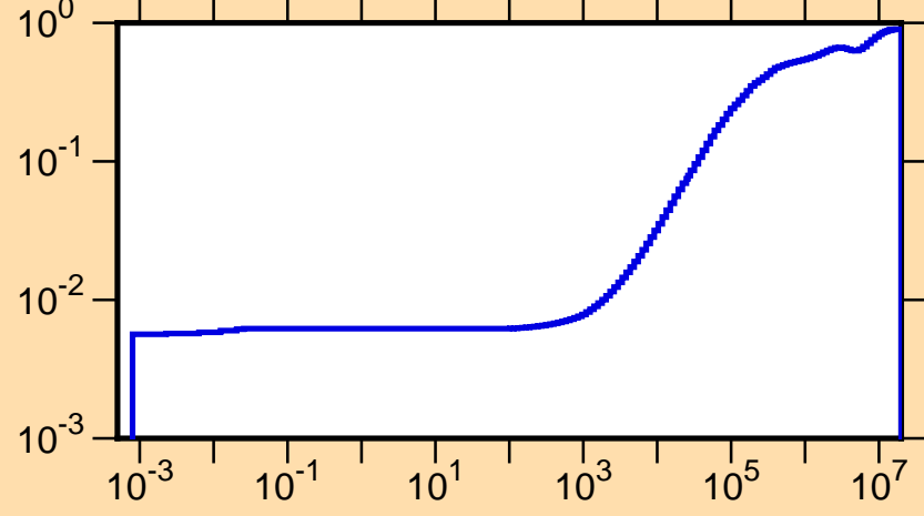
\mu vs. E for ^{120}\text{Sb}(\text{mt251})
