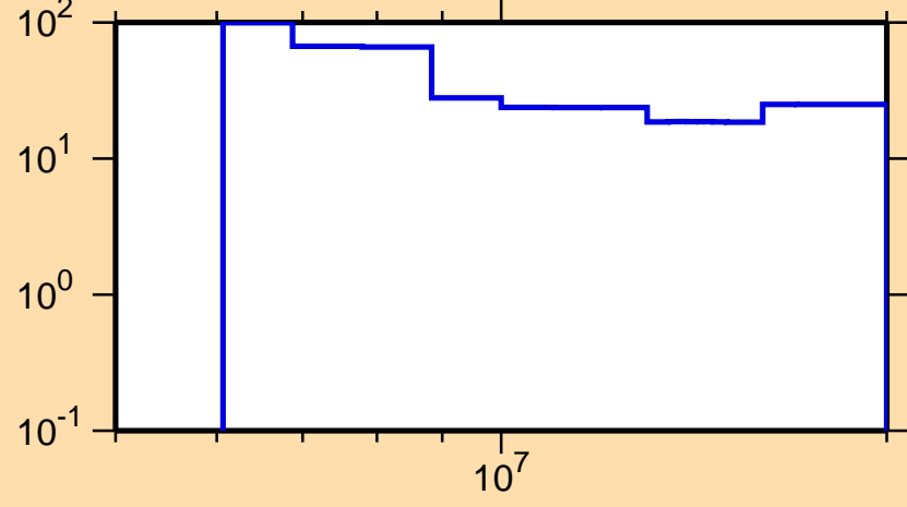
\Delta\sigma/\sigma vs. E for ^{120}\text{Sb}(n,2n)
