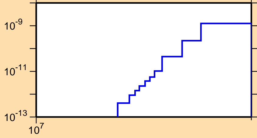
\sigma vs. E for ^{120}\text{Sb}(n,p\alpha)
