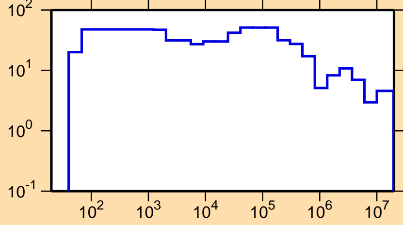
\Delta\sigma/\sigma vs. E for ^{120}\text{Sb}(n,\text{tot.})
