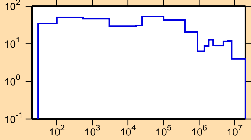
\Delta\sigma/\sigma vs. E for ^{120}\text{Sb}(n,\text{el.})
