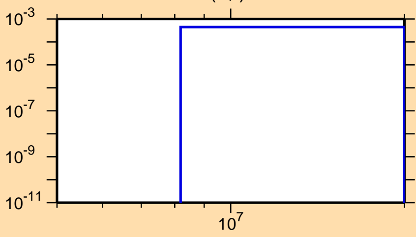
\sigma vs. E for ^{120}\text{Sb}(n,t)
