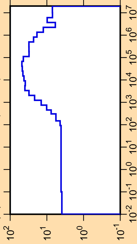
\Delta\mu/\mu vs. E for ^{121}\text{Sb}(\text{mt251})
