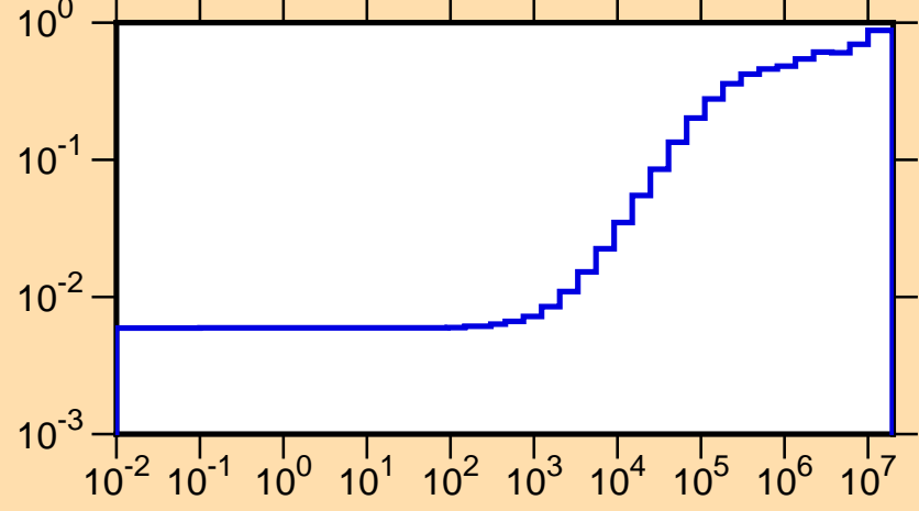
\mu vs. E for ^{121}\text{Sb}(\text{mt251})
