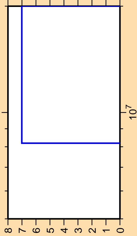
\Delta\sigma/\sigma vs. E for ^{121}\text{Sb}(n,2n)
