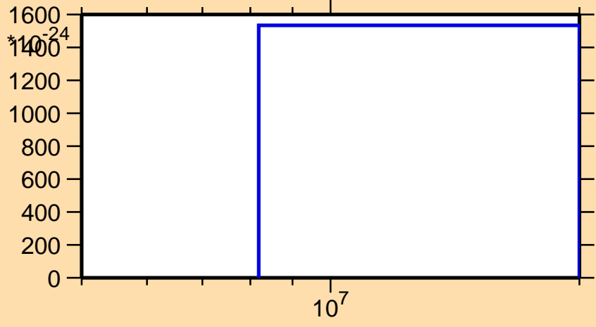
\sigma vs. E for ^{121}\text{Sb}(\text{mt } 11)
