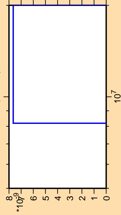
\Delta\sigma/\sigma vs. E for ^{121}\text{Sb}(\text{mt } 11)
