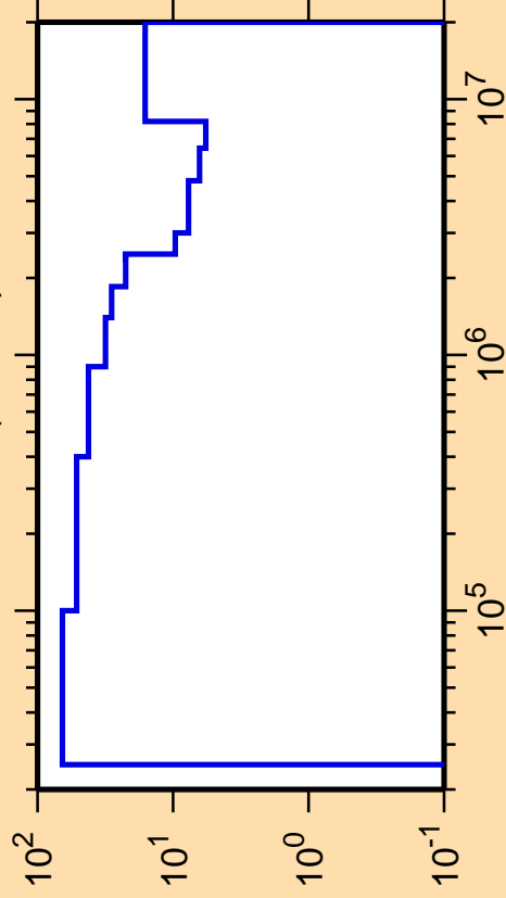
\Delta\sigma/\sigma vs. E for ^{121}\text{Sb}(n,\text{inel.})
