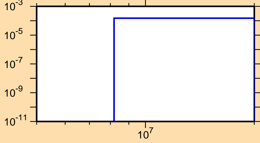
\sigma vs. E for ^{121}\text{Sb}(n,n\alpha)
