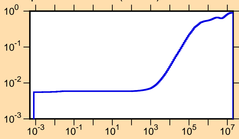
\mu vs. E for ^{122}\text{Sb}(\text{mt251})
