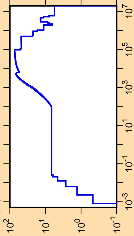
\Delta\mu/\mu vs. E for ^{122}\text{Sb}(\text{mt251})
