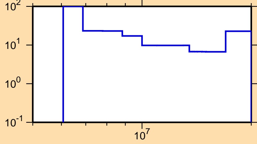
\Delta\sigma/\sigma vs. E for ^{122}\text{Sb}(n,2n)
