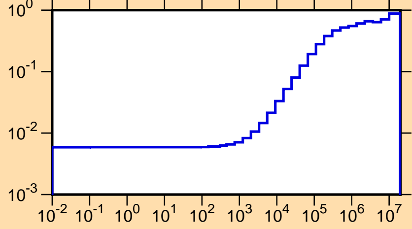
\mu vs. E for ^{122}\text{Sb}(\text{mt251})
