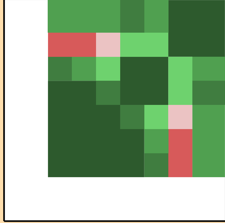
\sigma vs. E for ^{122}\text{Sb}(n,n\text{cont.})
