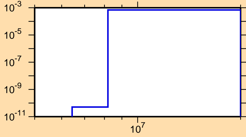
\sigma vs. E for ^{122}\text{Sb}(n,t)
