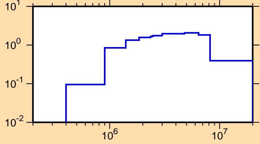
\sigma vs. E for ^{122}\text{Sb}(n,n\text{cont.})
