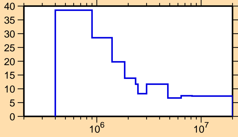
\Delta\sigma/\sigma vs. E for ^{122}\text{Sb}(n,n\text{onel.})
