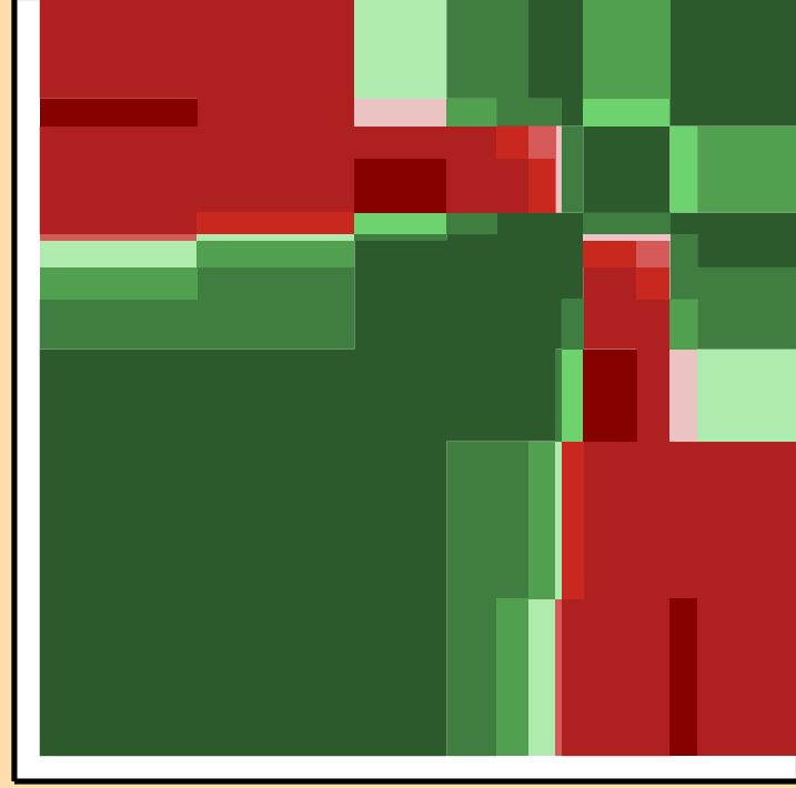
\sigma vs. E for ^{122}\text{Sb}(n,\text{inel.})
