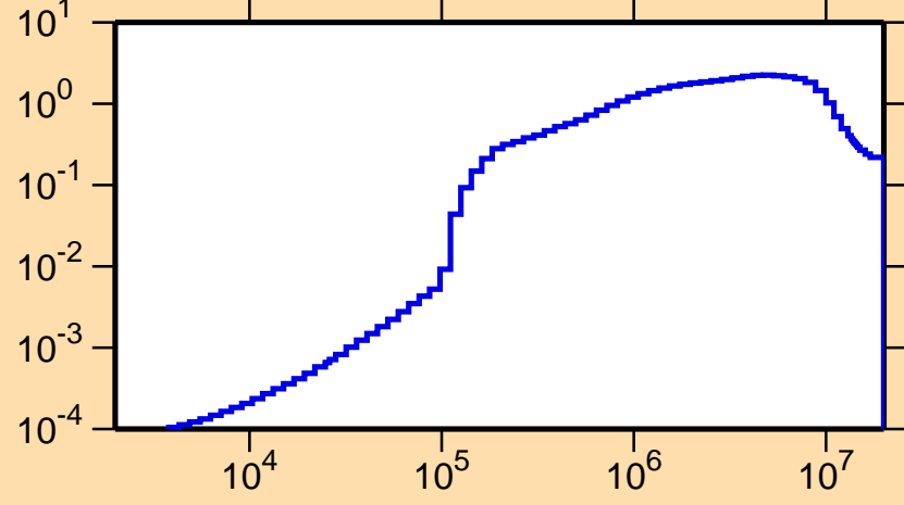
\sigma vs. E for ^{122}\text{Sb}(n,\text{inel.})
