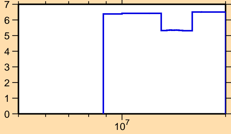
\Delta\sigma/\sigma vs. E for ^{123}\text{Sb}(n,\text{nonel.})
