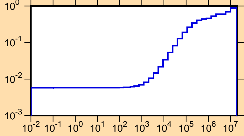
\mu vs. E for ^{123}\text{Sb}(\text{mt251})
