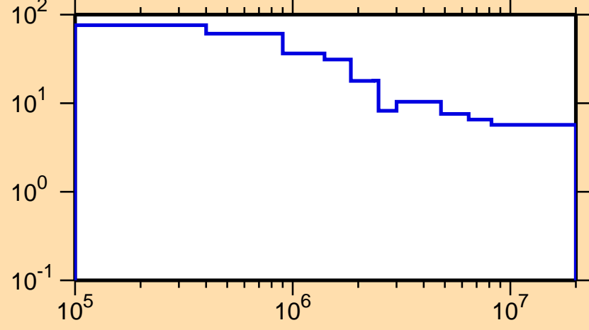
\Delta\sigma/\sigma vs. E for ^{123}\text{Sb}(n,\text{nonel.})
