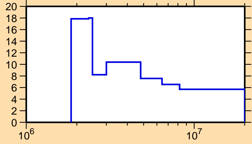
\Delta\sigma/\sigma vs. E for ^{123}\text{Sb}(n,n\text{onel.})
