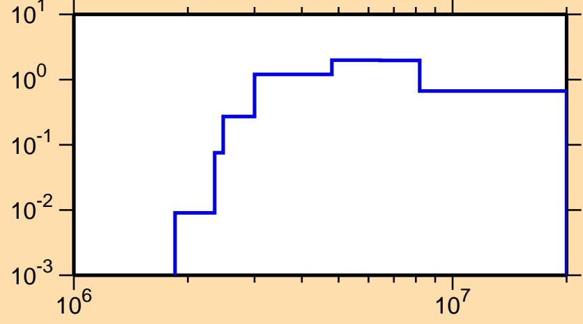
\sigma vs. E for ^{123}\text{Sb}(n,n\text{cont.})
