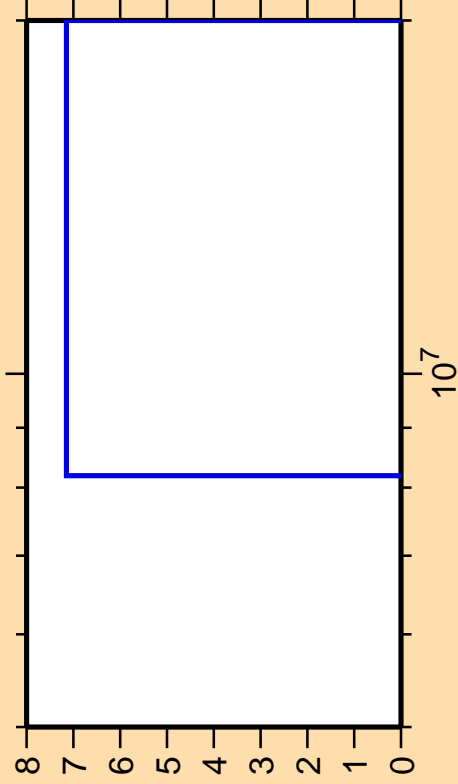
\Delta\sigma/\sigma vs. E for ^{123}\text{Sb}(n,2n)
