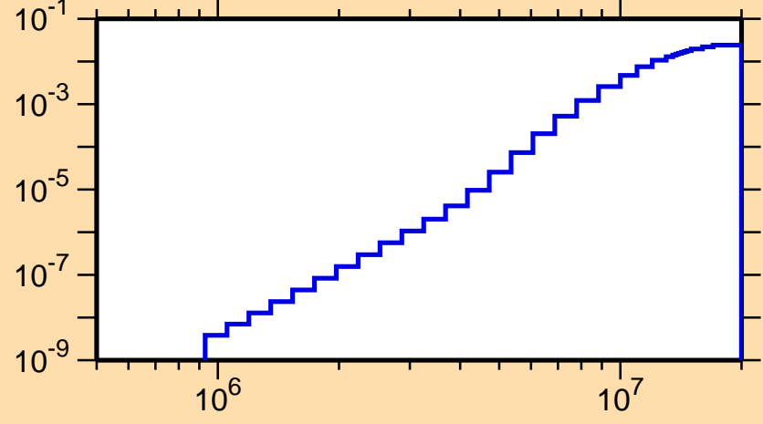
\sigma vs. E for ^{124}\text{Sb}(n,p)
