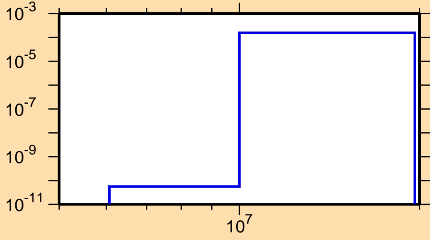
\sigma vs. E for ^{124}\text{Sb}(n,t)
