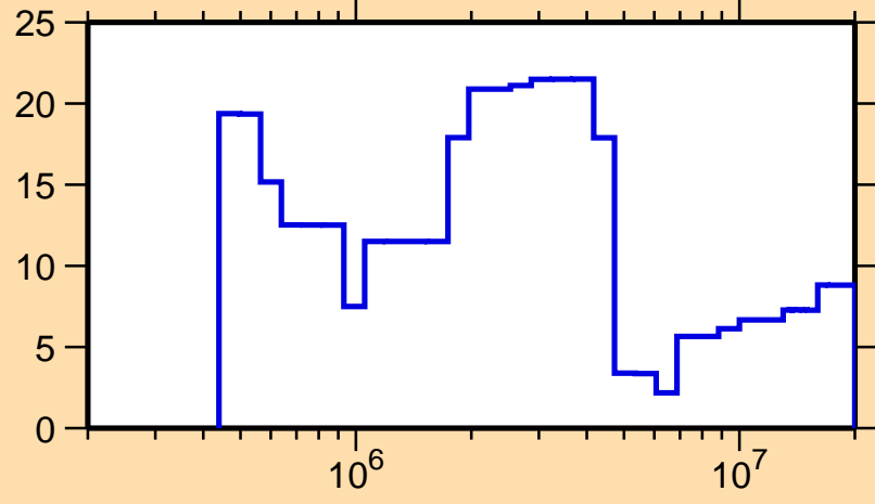
\Delta\sigma/\sigma vs. E for ^{124}\text{Sb}(n,el.)
