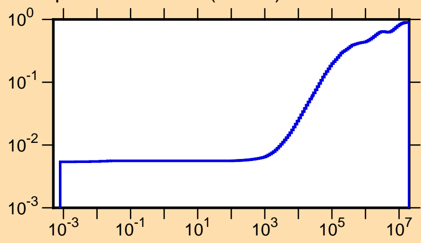
\mu vs. E for ^{125}\text{Sb}(\text{mt251})
