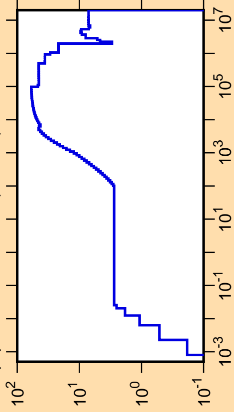
\Delta\mu/\mu vs. E for ^{125}\text{Sb}(\text{mt251})
