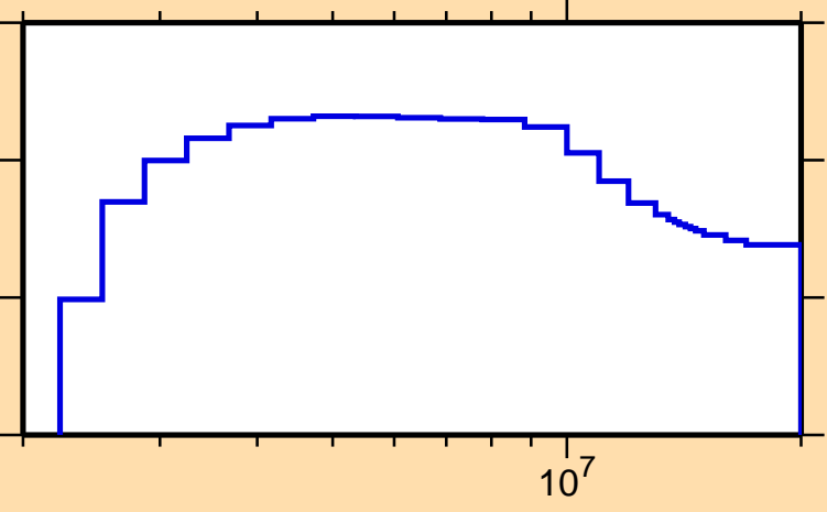
\sigma vs. E for ^{125}\text{Sb}(n,n\text{cont.})
