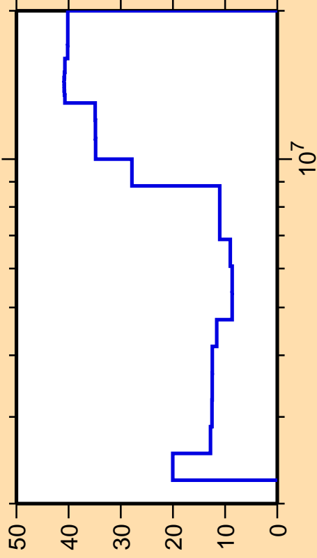
\sigma vs. E for ^{125}\text{Sb}(n,n\text{cont.})
