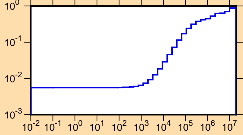
\mu vs. E for ^{125}\text{Sb}(\text{mt251})
