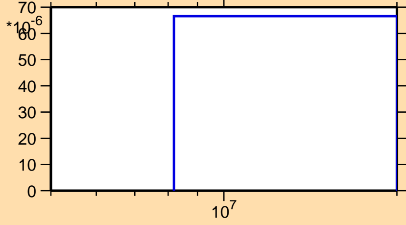
\sigma vs. E for ^{125}\text{Sb}(n,t)
