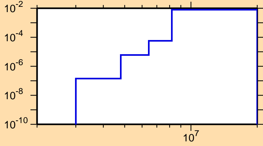
\sigma vs. E for ^{125}\text{Sb}(n,p)
