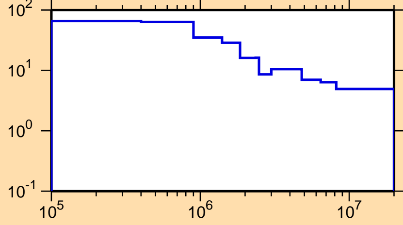
\Delta\sigma/\sigma vs. E for ^{125}\text{Sb}(n,\text{nonel.})
