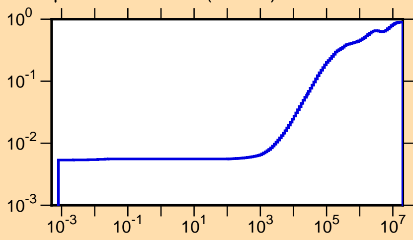
\mu vs. E for ^{126}\text{Sb}(\text{mt251})
