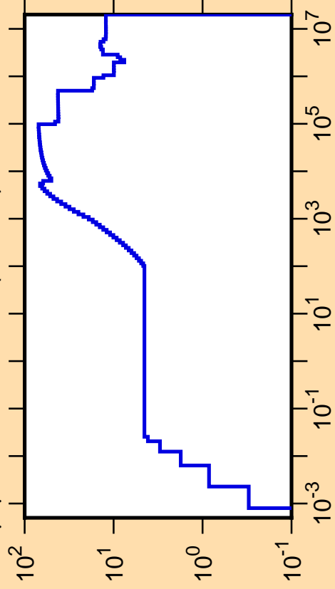
\Delta\mu/\mu vs. E for ^{126}\text{Sb}(\text{mt251})
