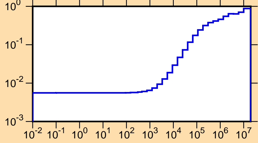
\mu vs. E for ^{126}\text{Sb}(\text{mt251})
