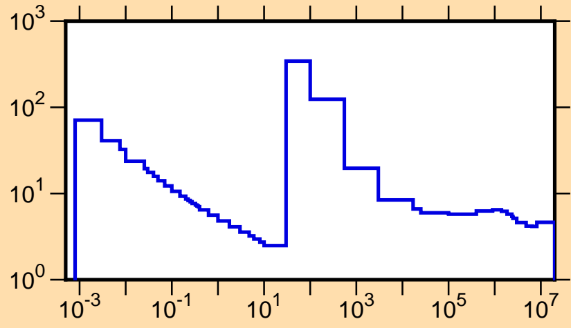
\sigma vs. E for ^{126}\text{Sb}(n,\text{tot.})
