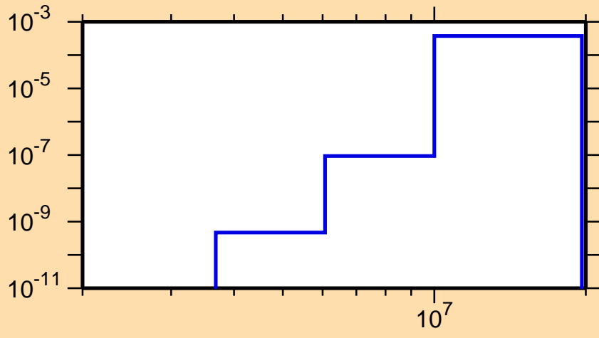
\sigma vs. E for ^{126}\text{Sb}(n,\alpha)
