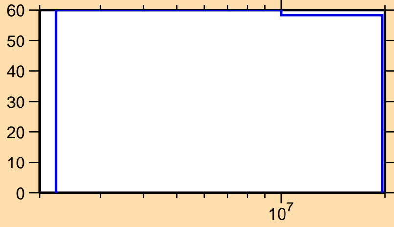
\Delta\sigma/\sigma vs. E for ^{126}\text{Sb}(n,p)
