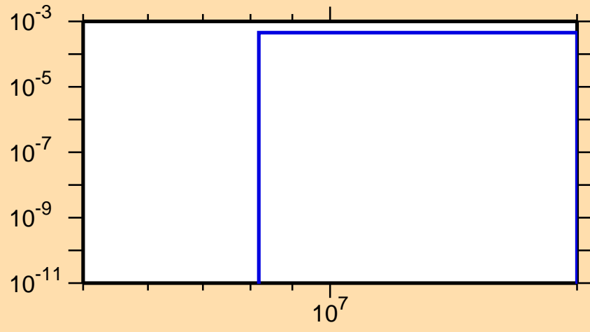
\sigma vs. E for ^{126}\text{Sb}(n,d)
