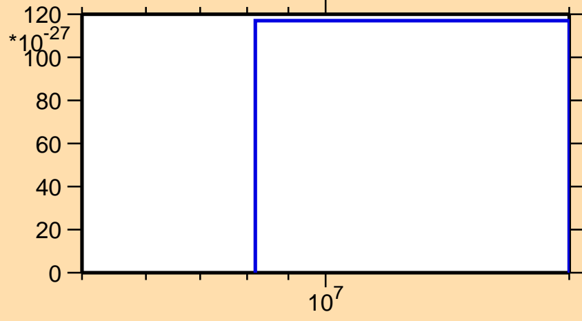
\sigma vs. E for ^{126}\text{Sb} (mt 11)
