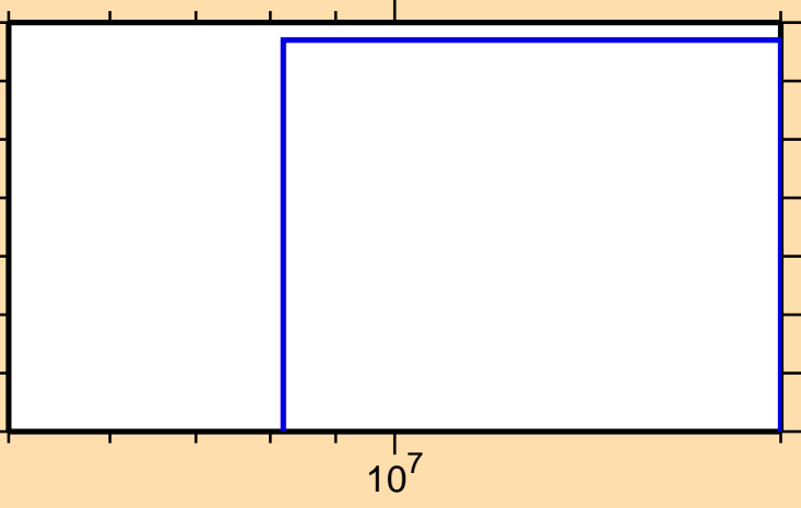
\sigma vs. E for ^{126}\text{Sb}(n,n\alpha)
