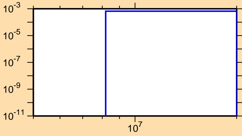
\sigma vs. E for ^{126}\text{Sb}(n,np)
