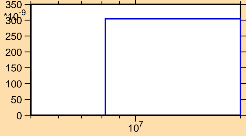
\sigma vs. E for ^{126}\text{Sb}(n,\text{nd})
