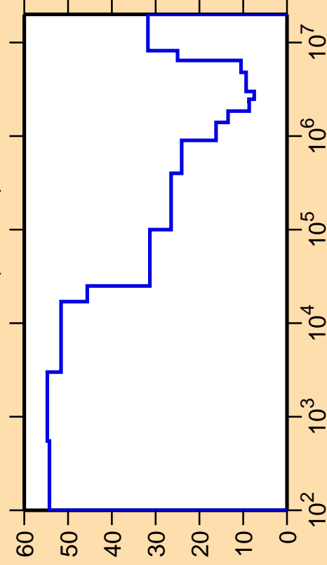
\Delta\sigma/\sigma vs. E for ^{126}\text{Sb}(n,\text{inel.})
