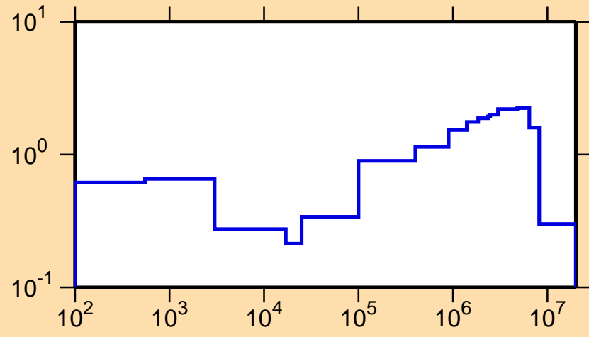
\sigma vs. E for ^{126}\text{Sb}(n,\text{inel.})
