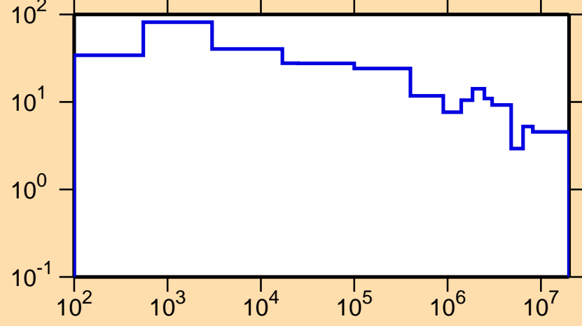
\Delta\sigma/\sigma vs. E for ^{126}\text{Sb}(n,\text{tot.})
