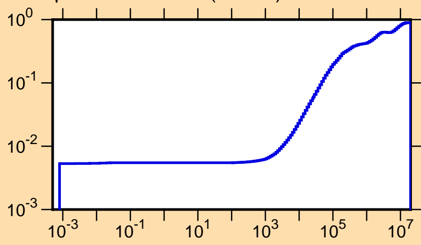
\mu vs. E for ^{127}\text{Sb}(\text{mt251})
