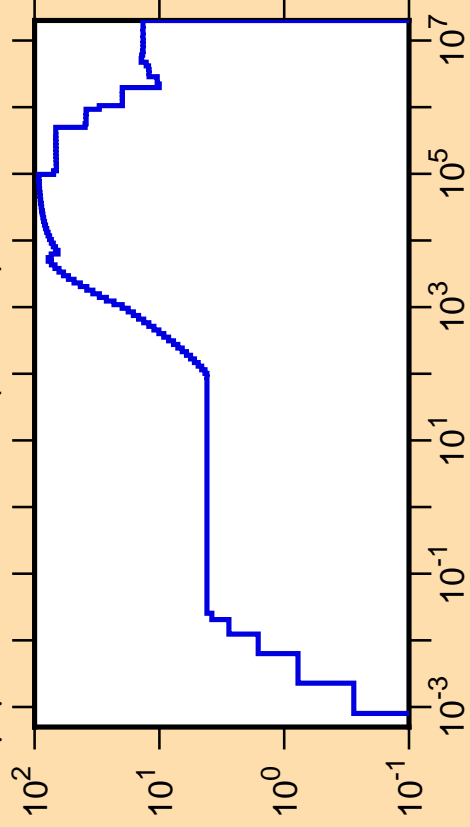
\Delta\mu/\mu vs. E for ^{127}\text{Sb}(\text{mt251})
