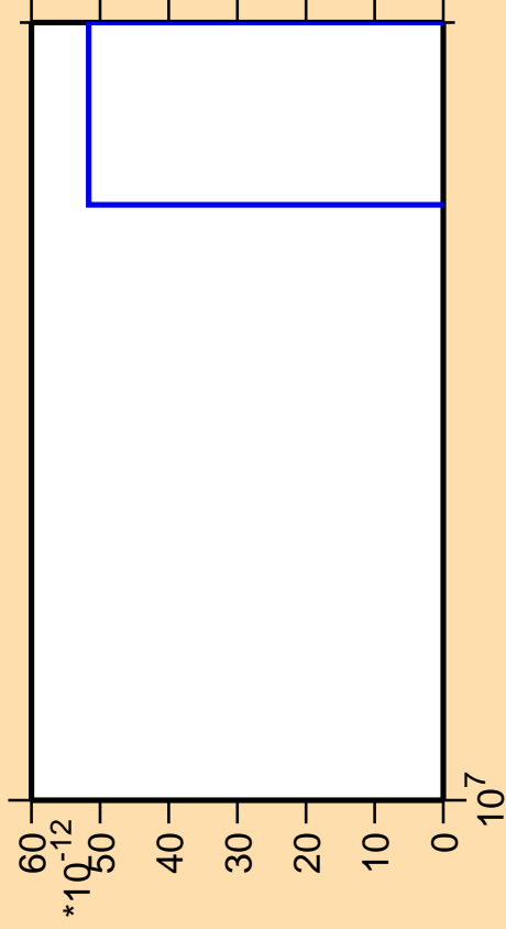
\Delta\sigma/\sigma vs. E for ^{127}\text{Sb} (mt 11)
