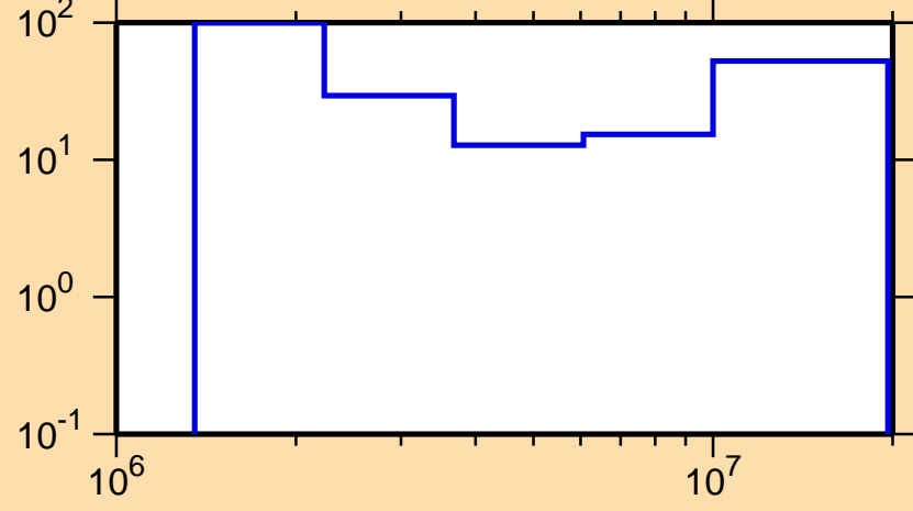
\Delta\sigma/\sigma vs. E for ^{127}\text{Sb}(n,n\text{cont.})
