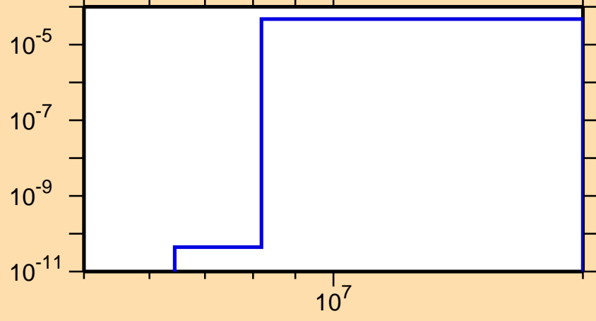
\sigma vs. E for ^{127}\text{Sb}(n,\alpha)
