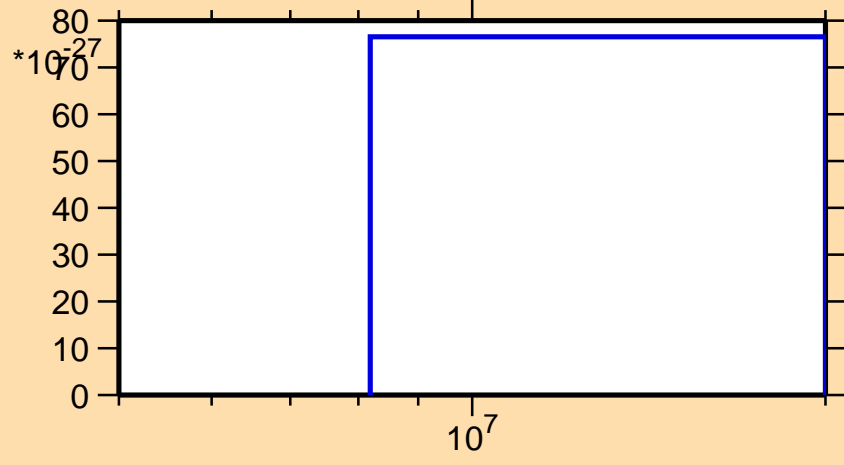
\sigma vs. E for ^{127}\text{Sb}(\text{mt } 11)
