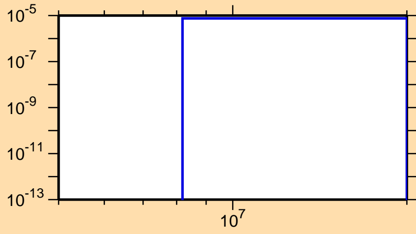
\sigma vs. E for ^{127}\text{Sb}(n,t)
