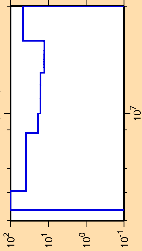
\Delta\sigma/\sigma vs. E for ^{128}\text{Sb}(n,2n)
