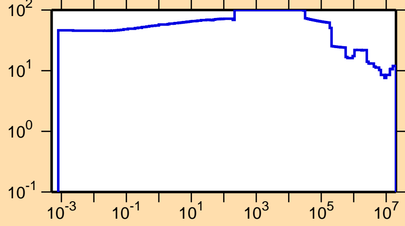
\Delta\sigma/\sigma vs. E for ^{128}\text{Sb}(n,\text{tot.})
