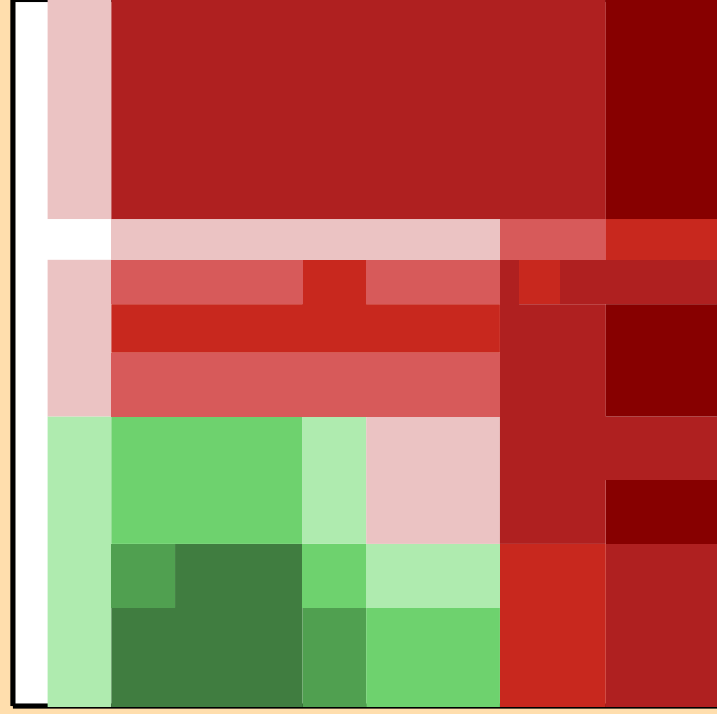
\Delta\sigma/\sigma vs. E for ^{128}\text{Sb}(n,2n)
