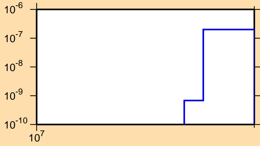
\sigma vs. E for ^{128}\text{Sb}(n,2np)
