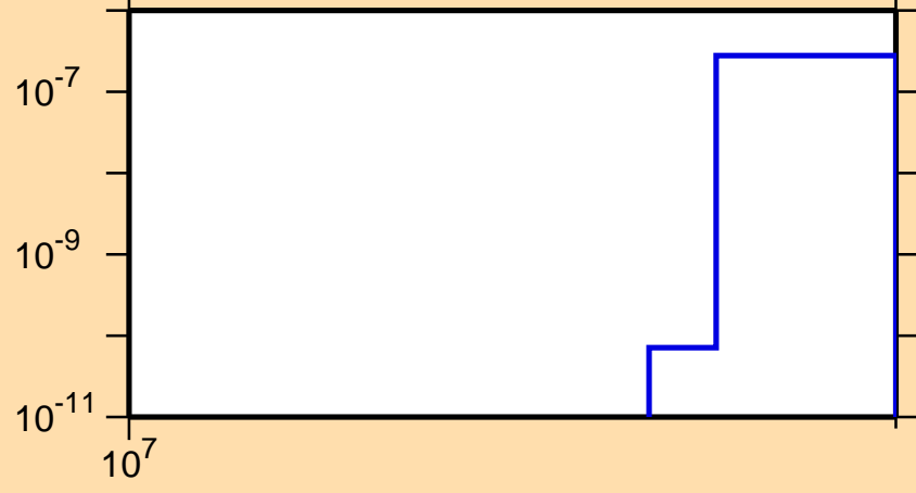
\sigma vs. E for ^{128}\text{Sb}(n,nt)
