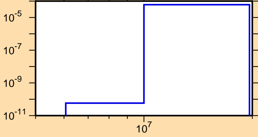
\sigma vs. E for ^{128}\text{Sb}(n,t)
