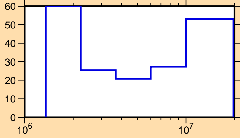
\Delta\sigma/\sigma vs. E for ^{128}\text{Sb}(n,ncont.)
