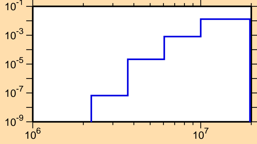
\sigma vs. E for ^{128}\text{Sb}(n,p)
