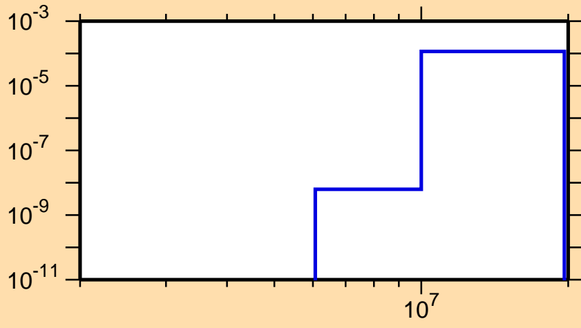
\sigma vs. E for ^{128}\text{Sb}(n,\alpha)
