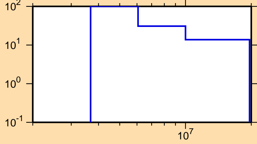
\Delta\sigma/\sigma vs. E for ^{128}\text{Sb}(n,2n)
