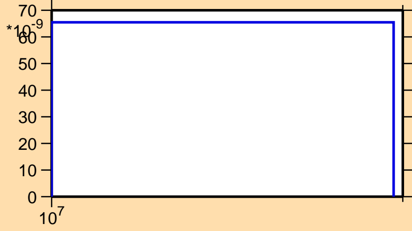
\sigma vs. E for ^{128}\text{Sb}(n,nd)
