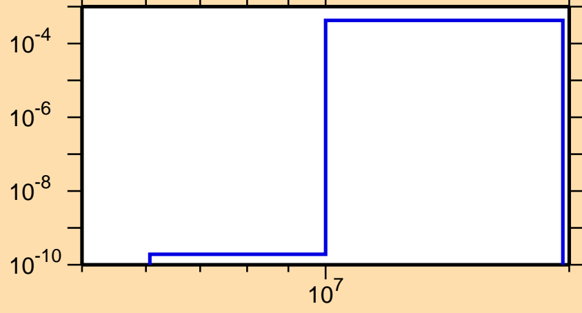
\sigma vs. E for ^{128}\text{Sb}(n,d)
