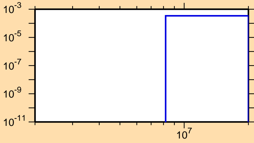
\sigma vs. E for ^{128}\text{Sb}(n,d)
